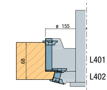
Raamprofilering
