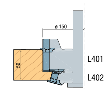
Raamprofilering
